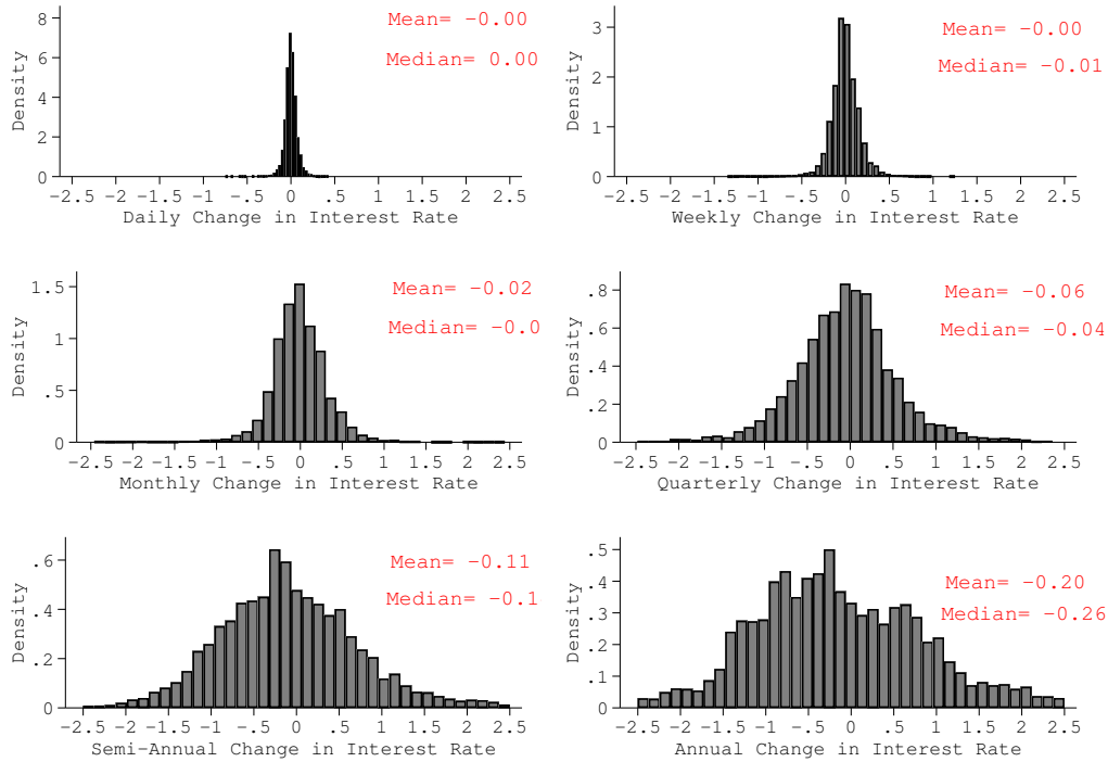
Figure 3: Distribution of Interest Rate Changes at Varying Frequencies
